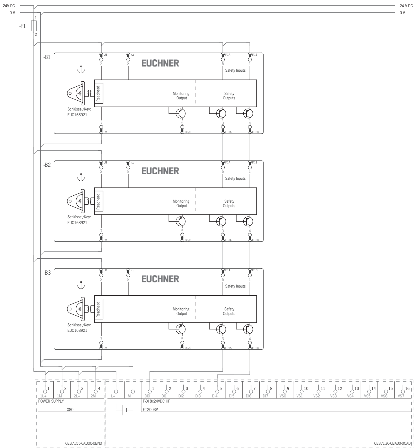
Fig. 2: Connection example for series connection with wiring in the control cabinet (principle of operation)
