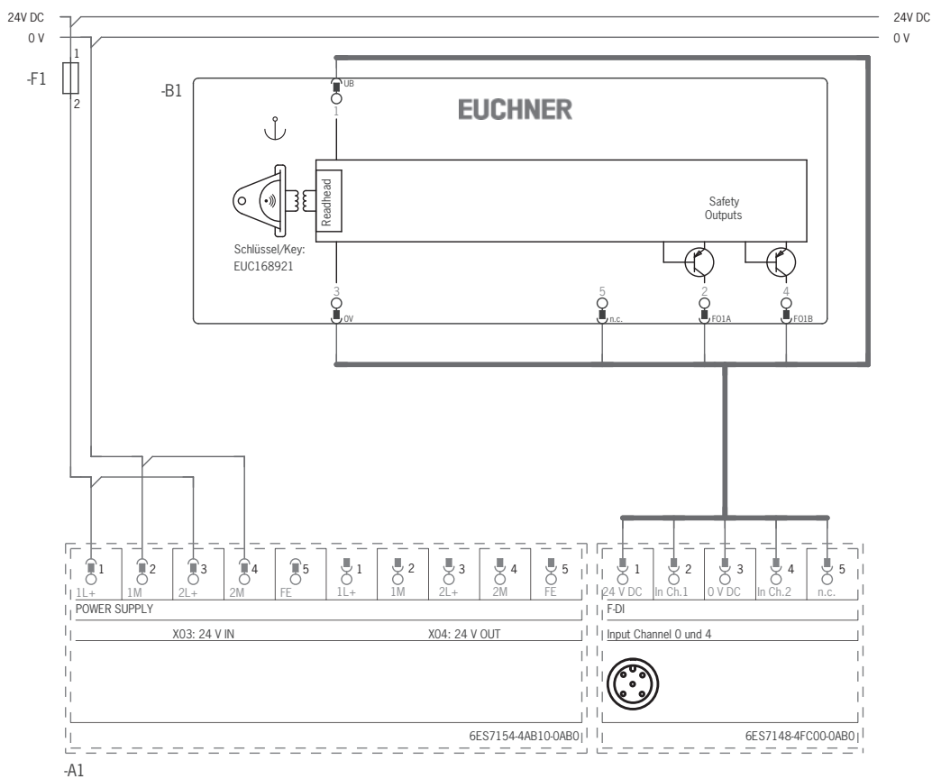
Fig. 1: Connection example for separate operation of an MSM-1-K-CKS2BP/BR-FLX-... on a safe IP67 peripheral module (principle of operation)
