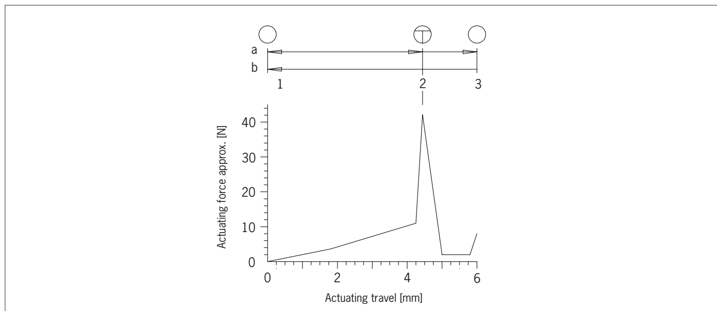
Fig. 3: Diagram of actuating force as a function of actuating travel
