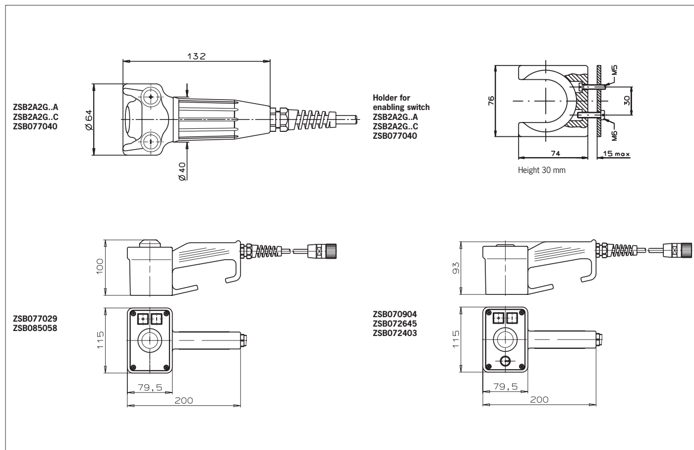
Fig. 1: Dimension drawing for enabling switch ZSA and holder for enabling switch ZSA
