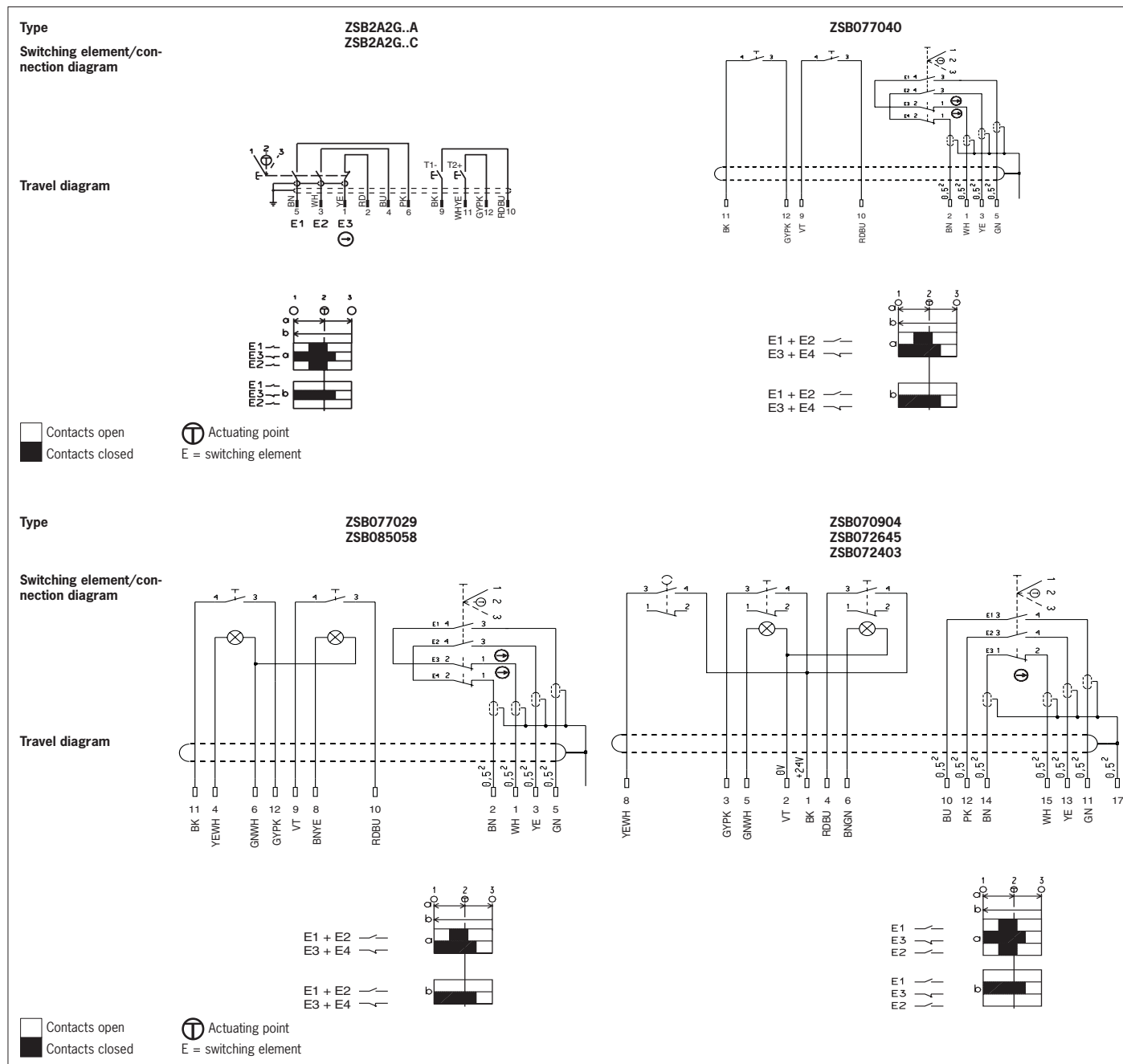
Fig. 2: Function of the switching elements and wiring diagrams
