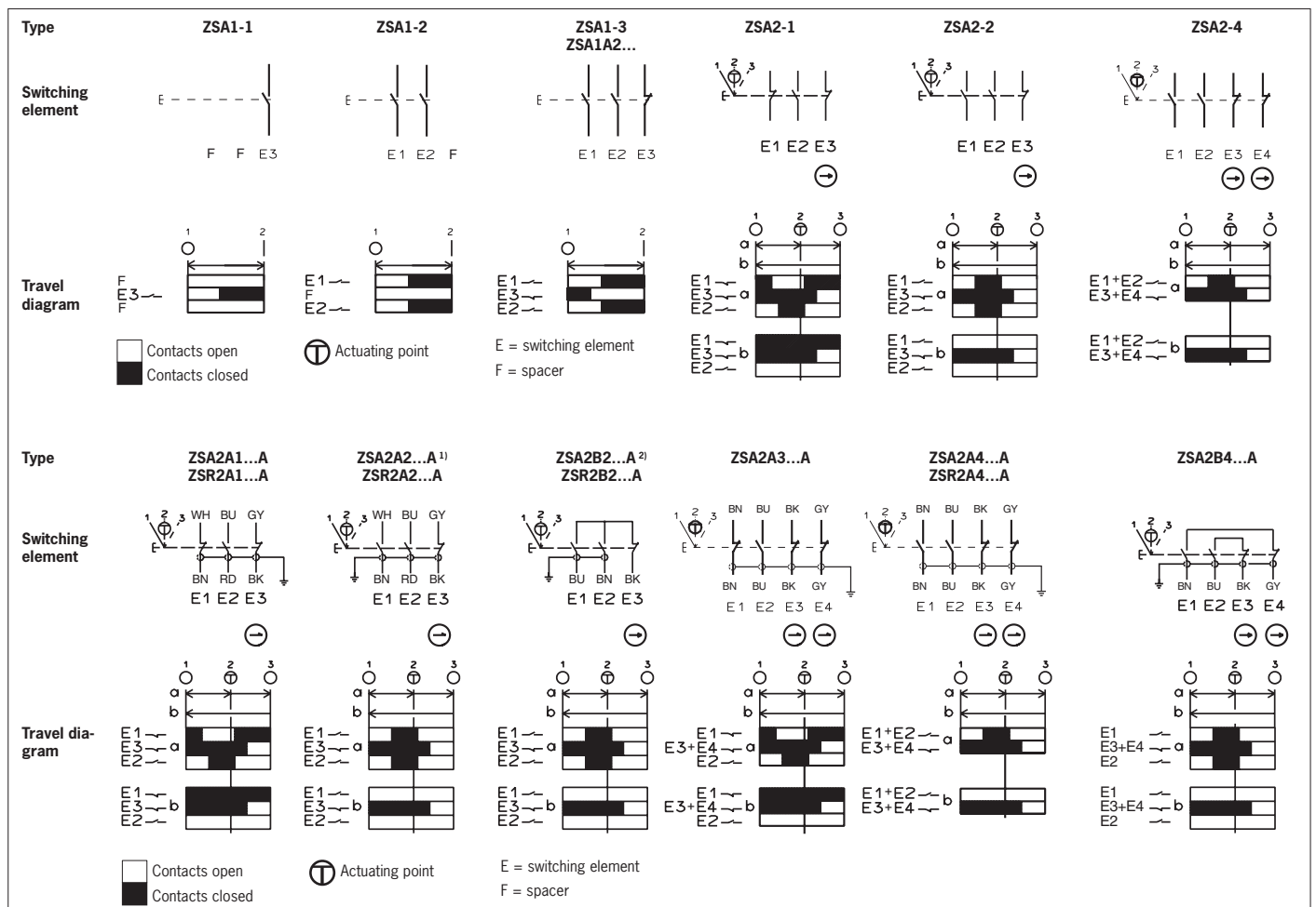
Fig. 1: Function of the switching elements (only for ZSA/ZSR with flying lead; see data sheet for plug)
