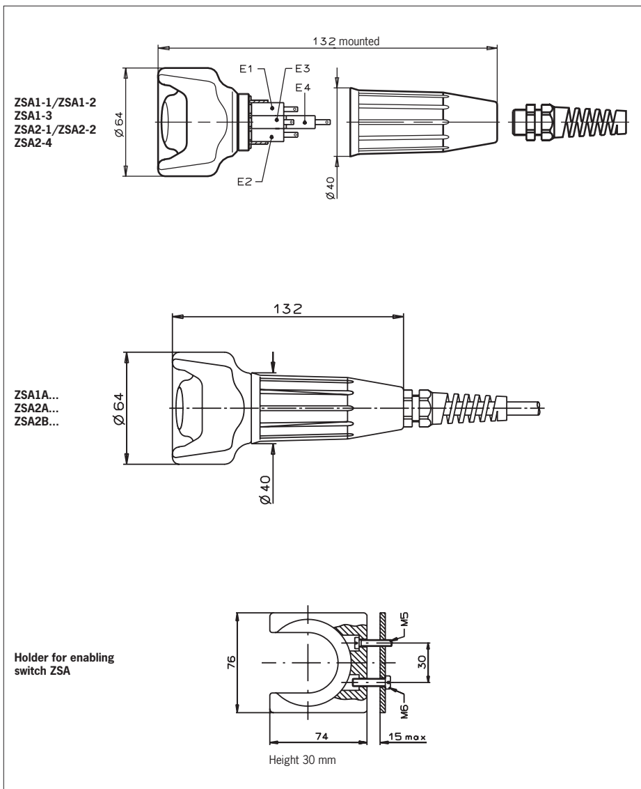
Fig. 2: Dimension drawing for enabling switch ZSA and holder for enabling switch ZSA
