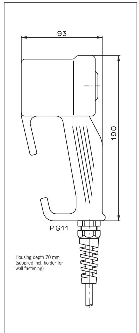
Fig. 3: Dimension drawing for enabling switch ZSR
