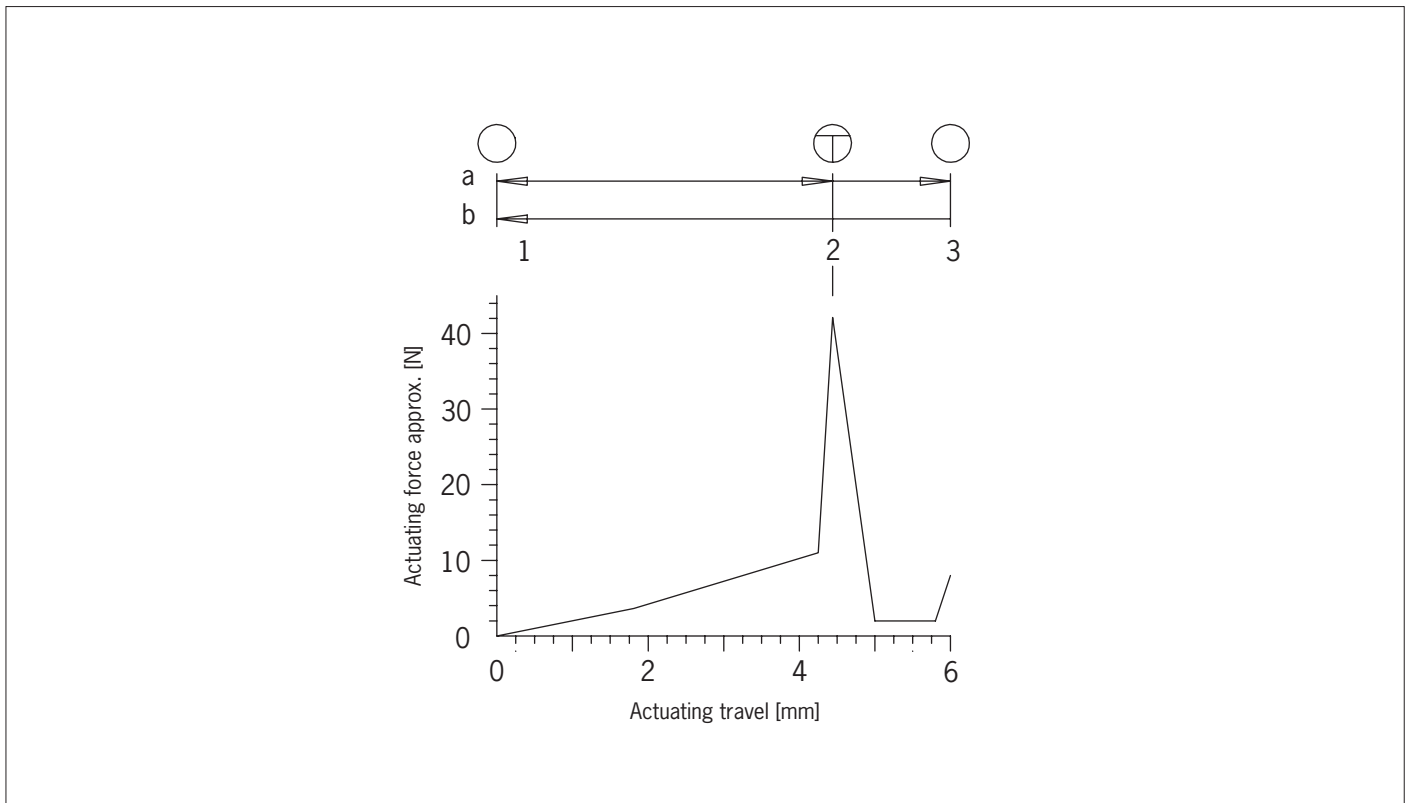
Fig. 4: Diagram of actuating force as a function of actuating travel
